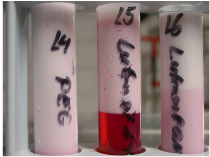
(b) Lutensol
